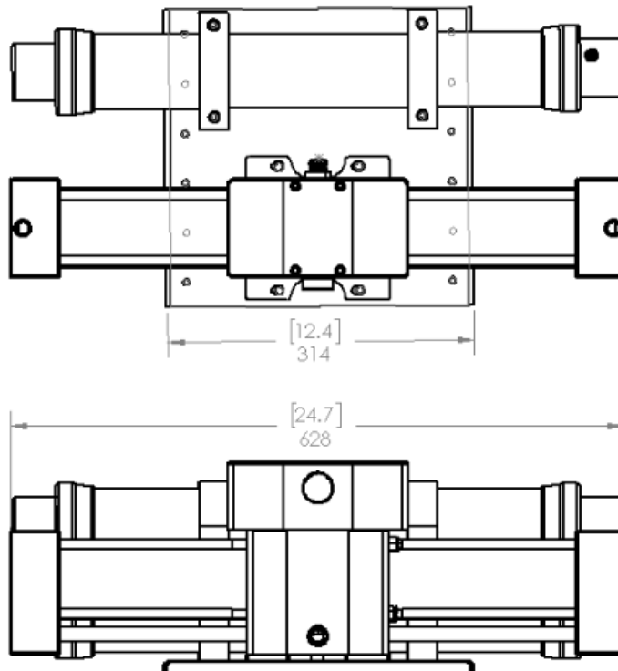
Figure 36: High Pressure Module, Duel 21" Membrane
