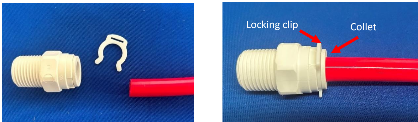
Figure 20: Fitting, Locking Clip & Tubing Installation
