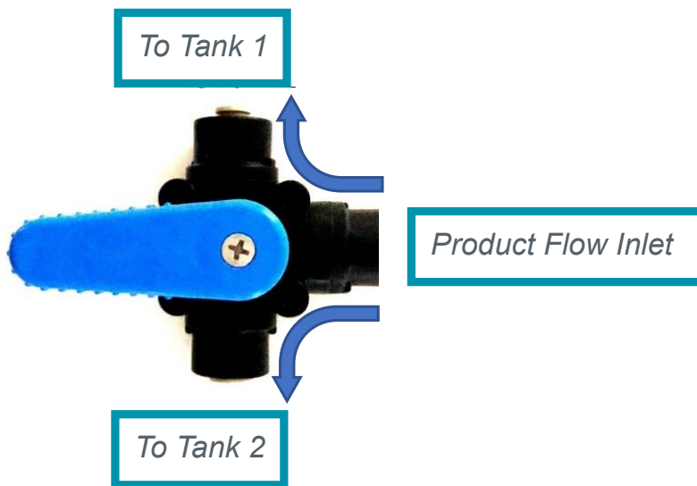
Figure 16: Optional Tank fill Selector Valve (Owner Supplied)
