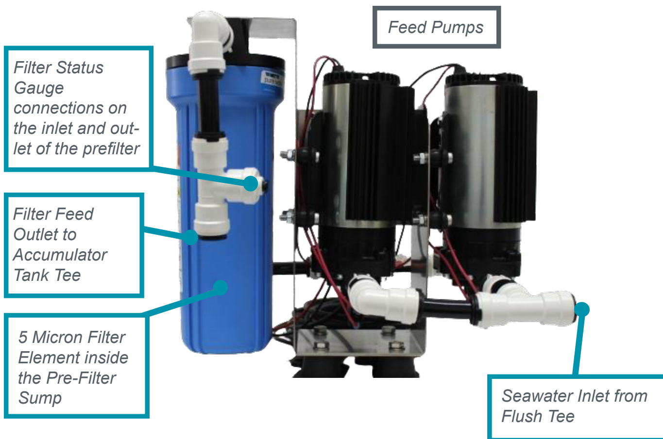
Figure 6: Feed Pump Assembly
